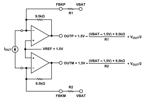
Figure 47. Decreasing the Output Common-Mode Voltage
