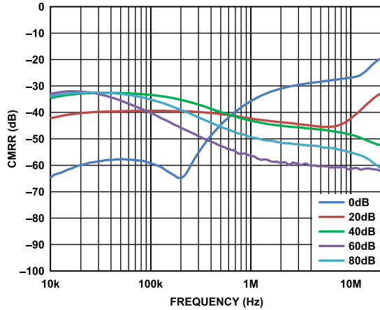
Figure 16. Common-Mode Rejection Ratio (CMRR) vs. Frequency over Gain, Offset Null On, Referred to Input
