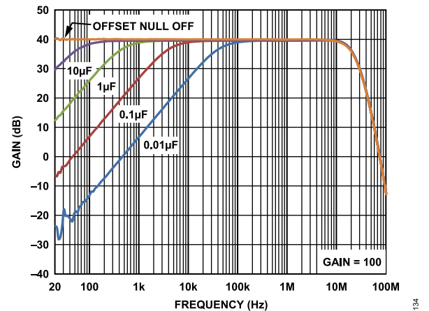
Figure 33. Offset Null Bandwidth vs. Offset Null Capacitor
