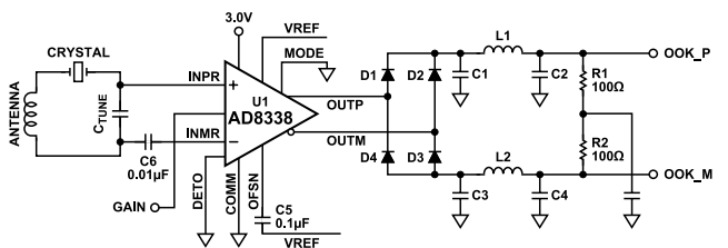
Figure 49. Complete, Low Power OOK Receiver
