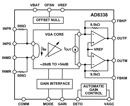
Figure 39. Block Schematic
