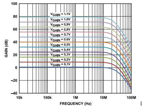
Figure 2. Gain vs. Frequency
