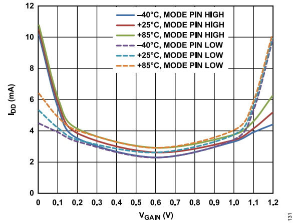
Figure 32. Supply Current vs. V_{GAIN}
