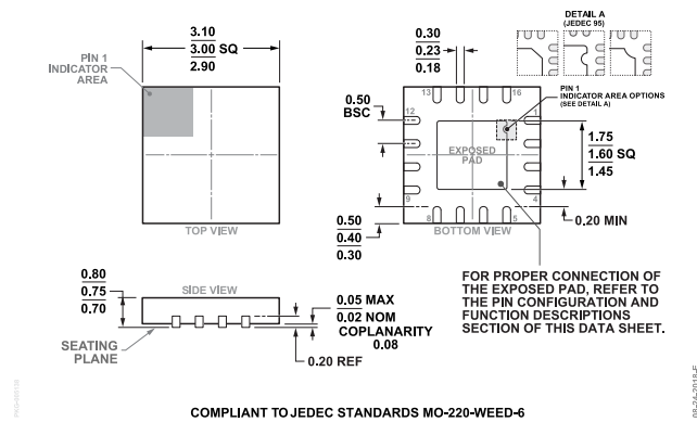
Figure 50. 16-Lead Frame Chip Scale Package [LFCSP] 3 mm x 3 mm Body and 0.75 mm Package Height (CP-16-22) Dimensions shown in millimeters
